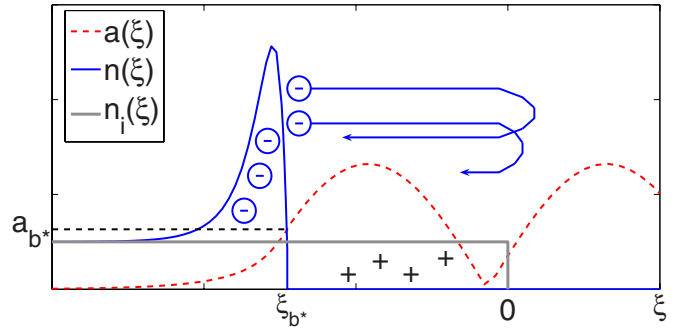
FIG. 1. (Color online) Schematic of quasistationary model of laser-plasma interaction: spatial distributions of electromagnetic field a , electron n , and ion n_i densities.
