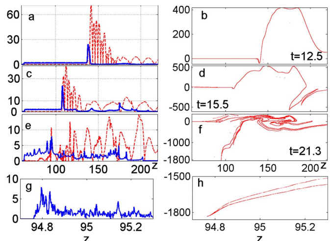
FIG. 4. (Color online) The same as in Fig. 2, but for the incident 5 fs Gaussian pulse with maximal amplitude a_0=60 . Data for the generated electron beam: (g) snapshot of the density distribution and (h) its detailed phase portrait.
