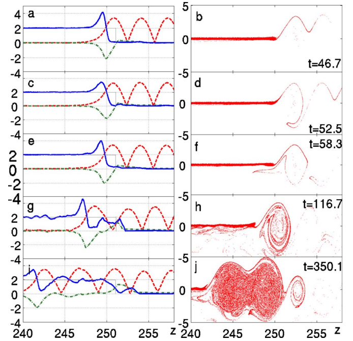
FIG. 2. (Color online) Space-time dynamics [(a), (c), (e), (g), and (i)] of the interaction of incident (on the right of the boundary) semibounded pulse of maximal amplitude a_0 = 1.7 with supercritical plasma n_o = 2 : distribution of electron density (continuous curve), ions (dotted curve), absolute value of vector potential (dashed curve), and longitudinal electric field (dot-dashed curve) at different moments of time. The corresponding phase portraits (longitudinal momentum in relativistic units along propagation direction) of the electrons are plotted on the right [(b), (d), (f), (h), and (j)].
