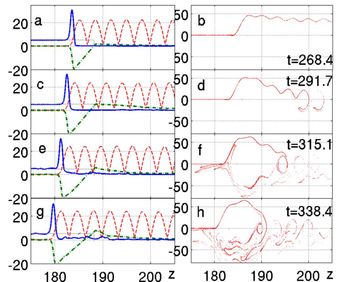
FIG. 3. (Color online) The same as in Fig. 2 but for a_0 = 12.8 and n_o = 5 .
